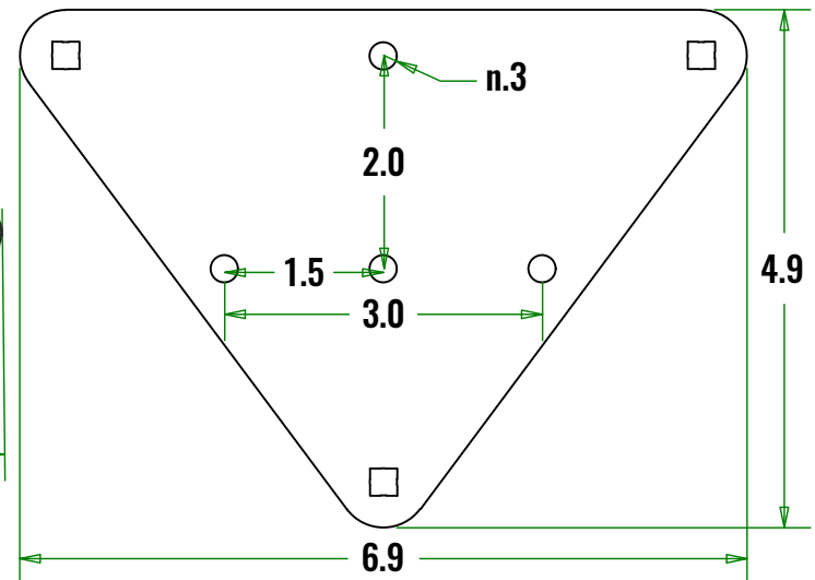
Talon Mounting Bracket
